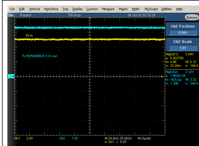
Fig7: TLV62569DRLR _P3V3_Vin Vout
