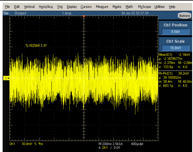
Fig8: TLV62569DRLR _P3V3_ripple
