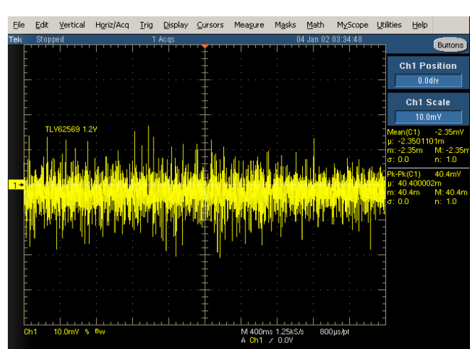
Fig6: TLV62569DRLR_P1V2_ripple
